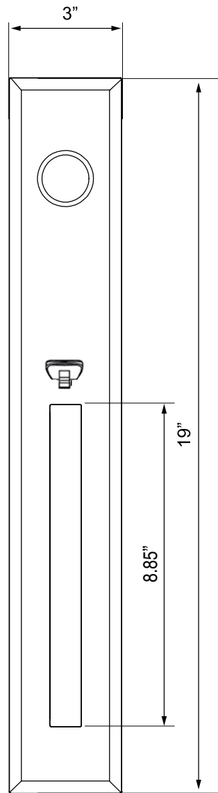
Front View
