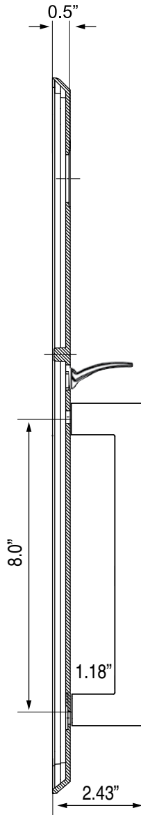
Side View
