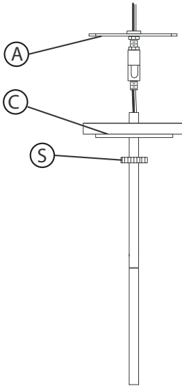
Drawing 1 – Stem Assembly
