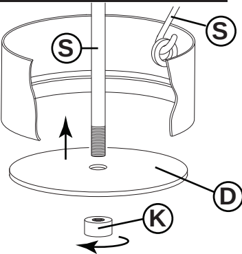
DRAWING 3 - FINAL ASSEMBLY
