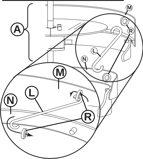
DRAWING 2 - FINAL ASSEMBLY
