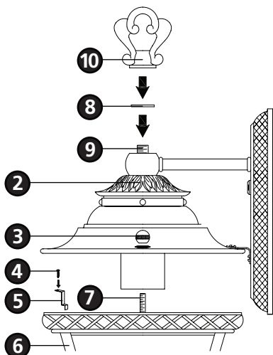
Drawing 3 - Fixture Assembly
