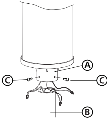
Drawing 2 - Lamping Fixture
