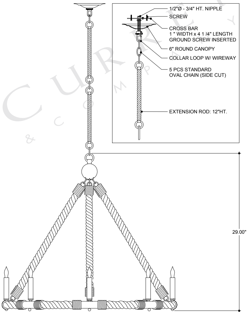
FRONT VIEW
