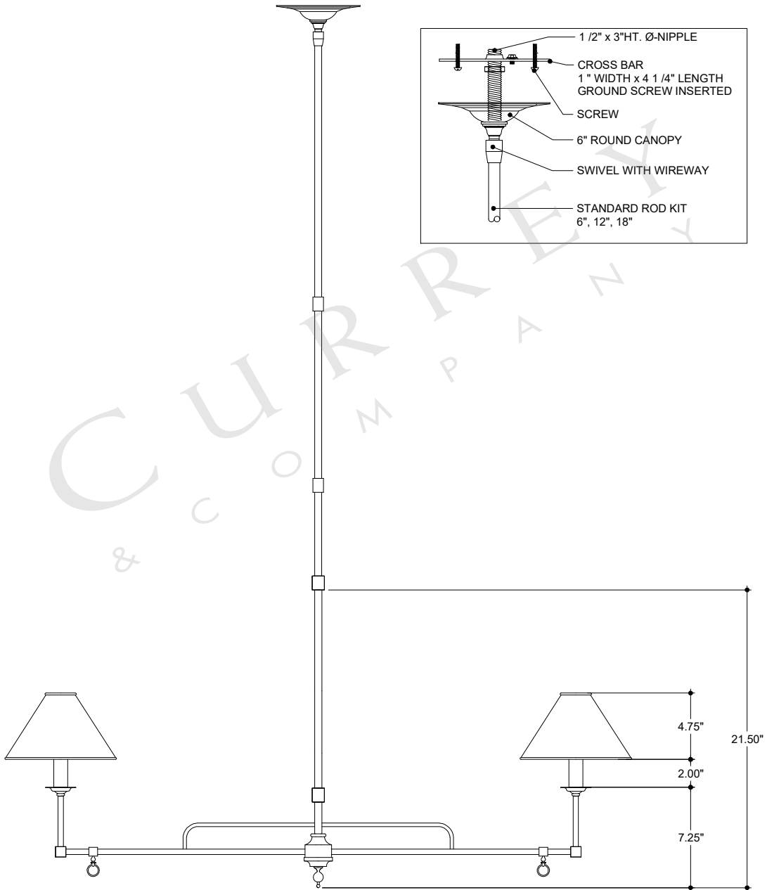
FRONT VIEW
