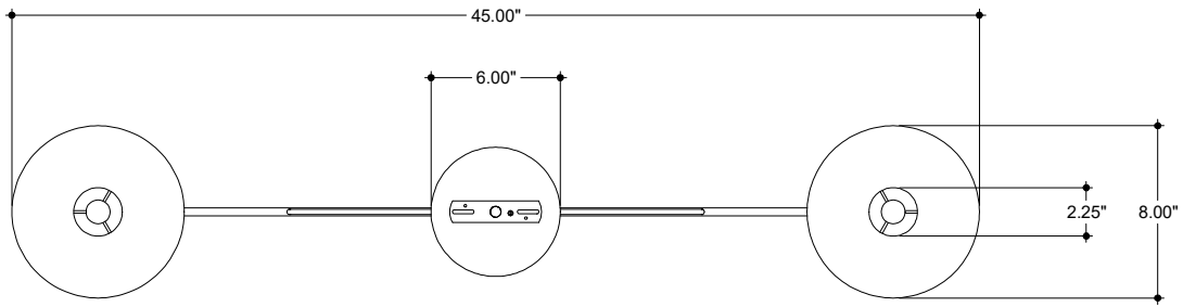
TOP VIEW
