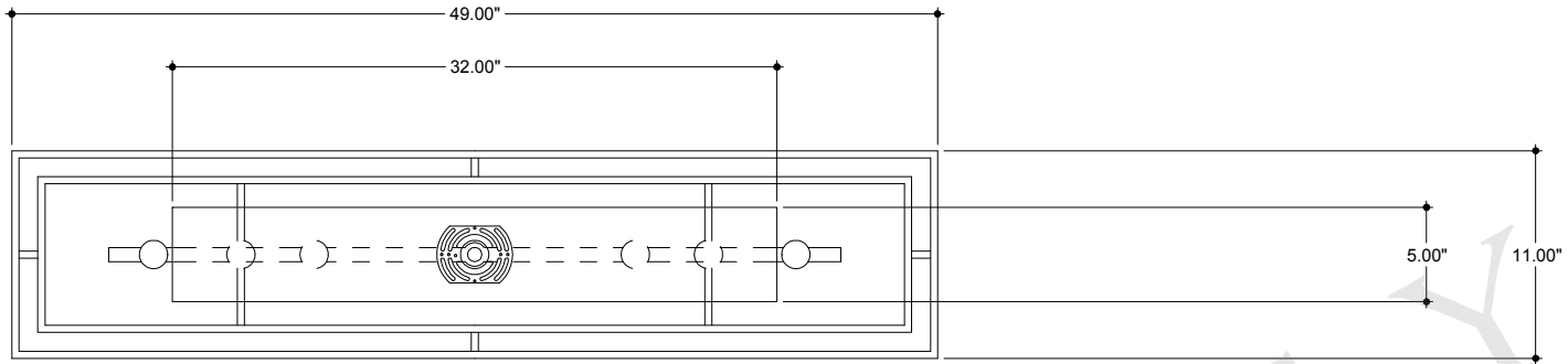
TOP VIEW
