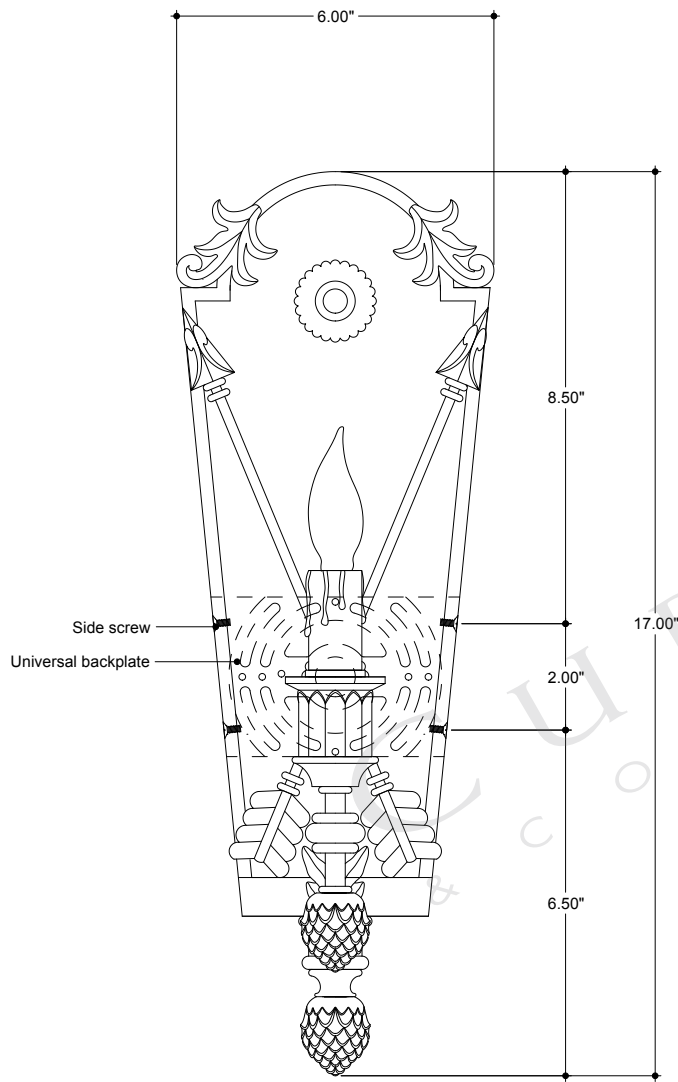
FRONT VIEW
